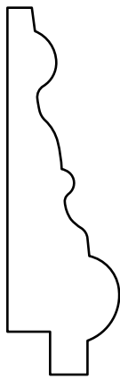
RHPC 5/8" x 2-1/8"
