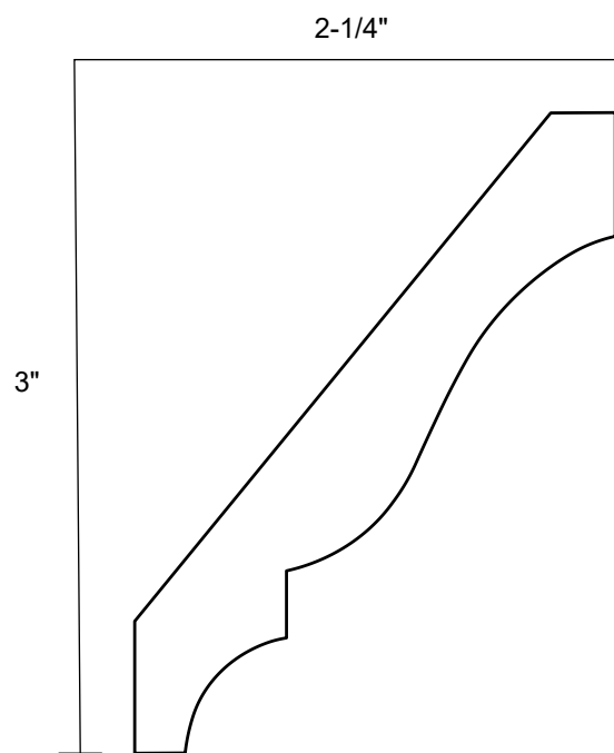
8009 9/16" x 3-5/8"
